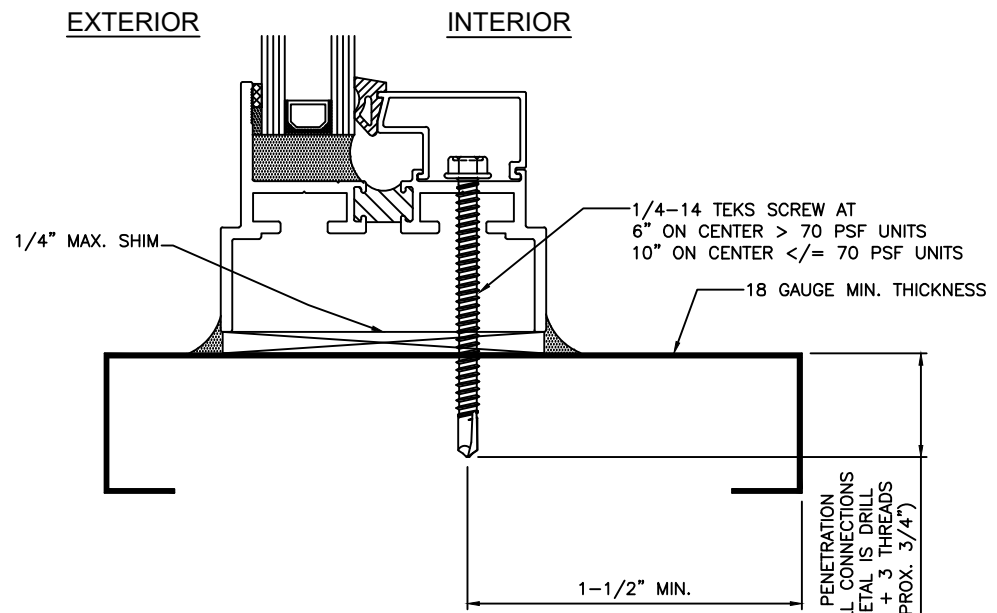
SECTION 1/1, 1/2 & 1/3 THROUGH FRAME TO STEEL STUD
