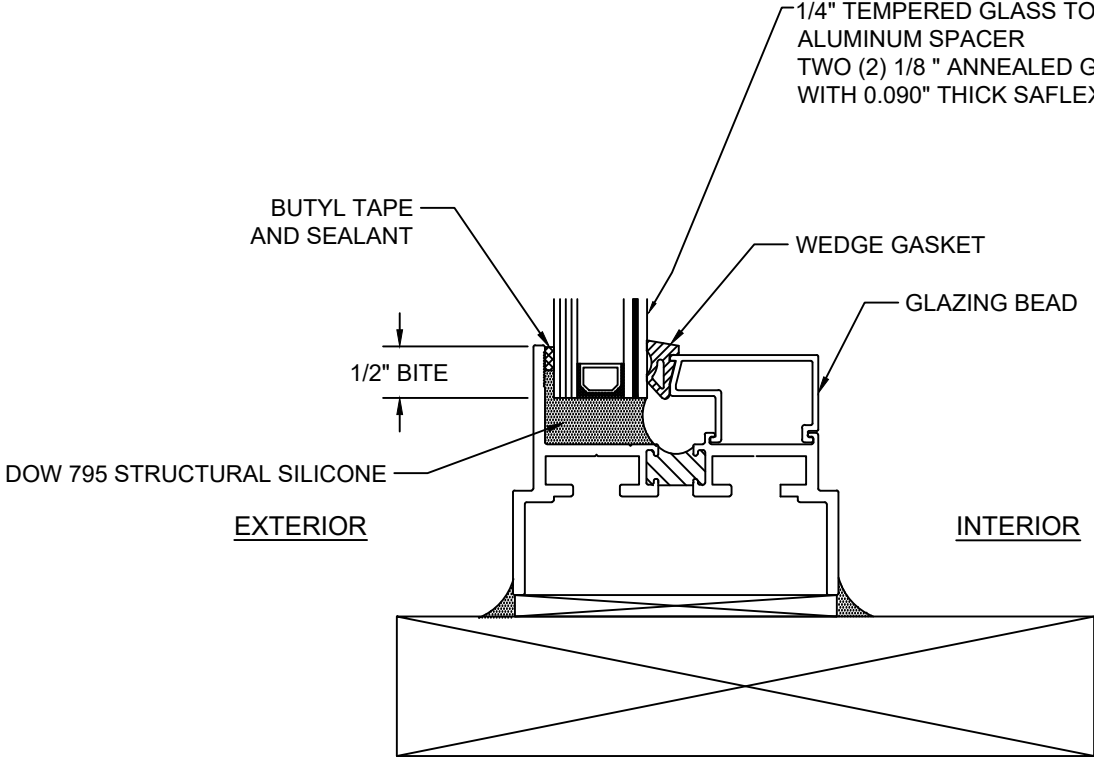
INSULATING GLASS GLAZING DETAIL
