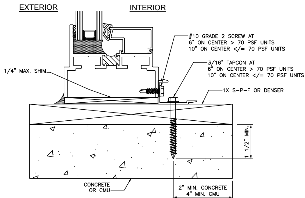
SECTION 1/1, 1/2 & 1/3 INSIDE CLIP & ANCHOR TO CONCRETE OR CMU WITH 1X BUCK STRIP
